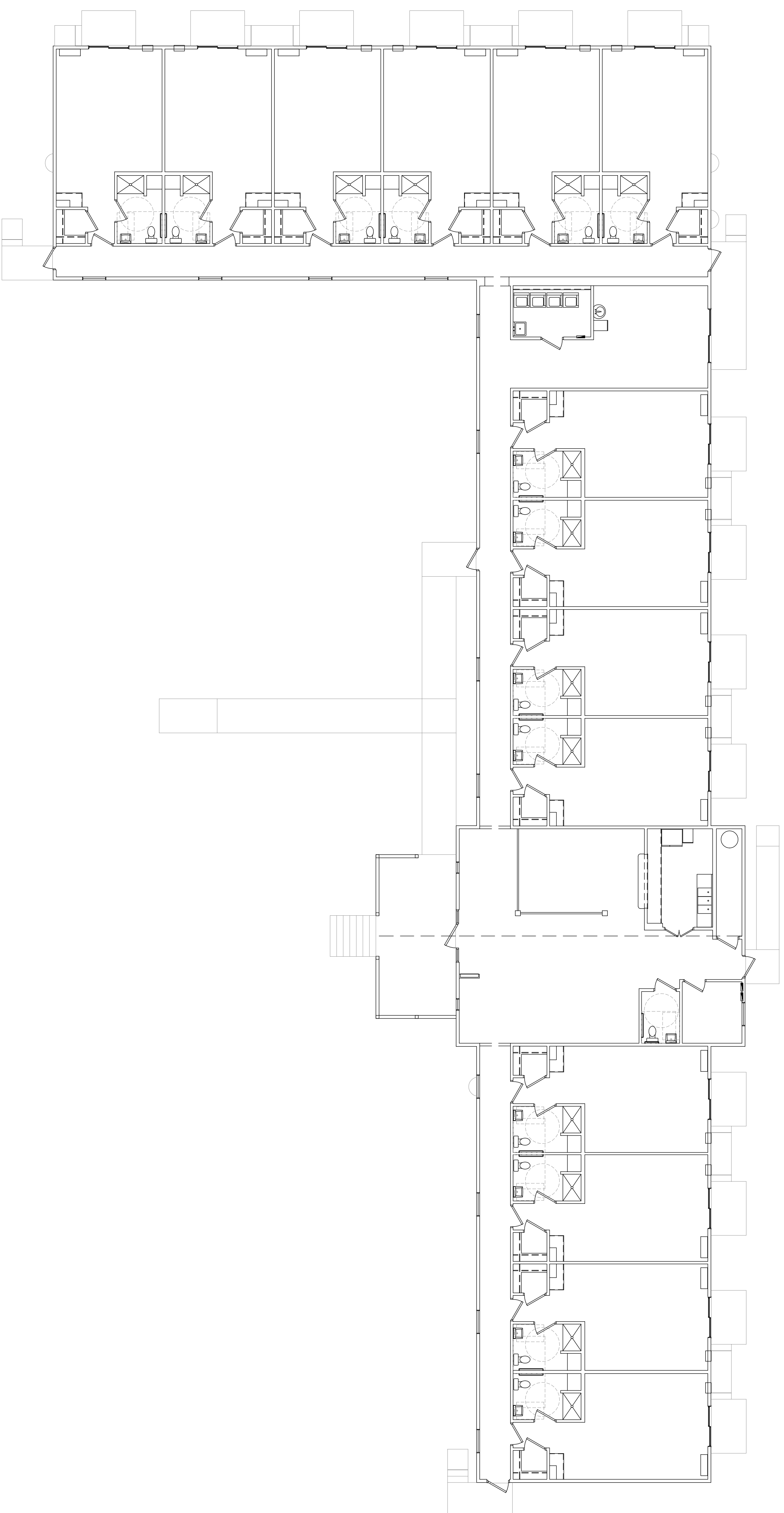
1 FLOOR PLAN - EXISTING SCALE: 1/8"=1'-0"
